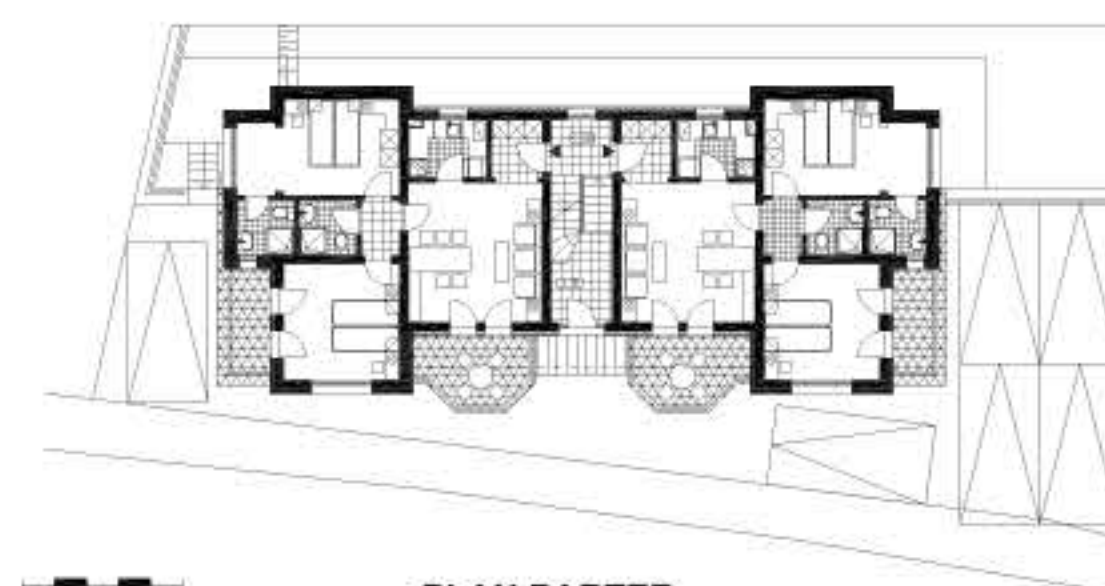
PLAN PARTER
